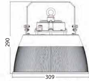
100W High Bay With PC Reflector
