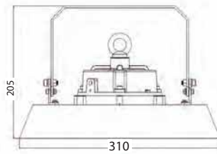
120W / 150W High Bay With Bracket
