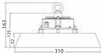
120W / 150W High Bay
