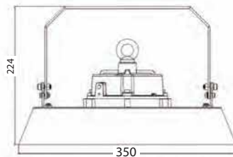
200W High Bay With Bracket
