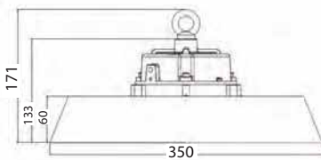
200W High Bay
