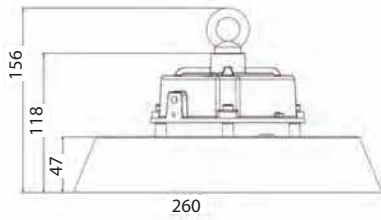
100W High Bay
