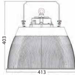
120W/150W High Bay With PC Reflector
